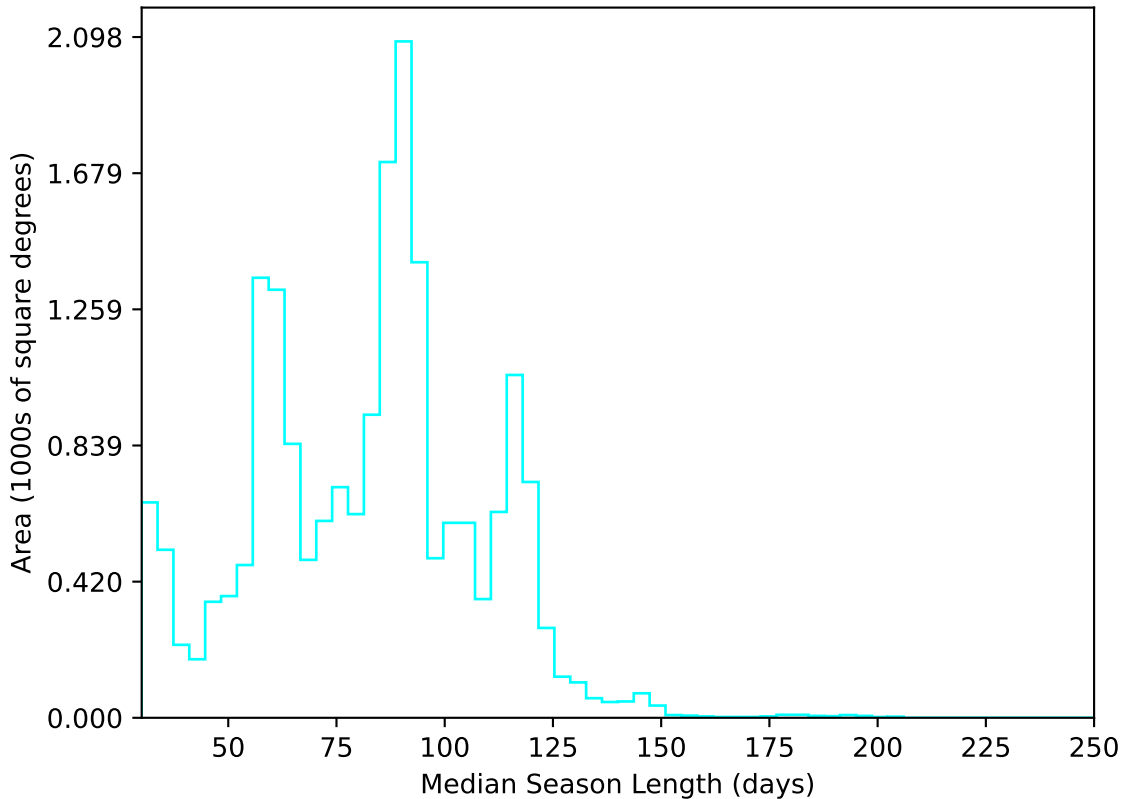
too_elab_r8_d3_griz_v3.4_10yrs All sky u band: Median Season Length
