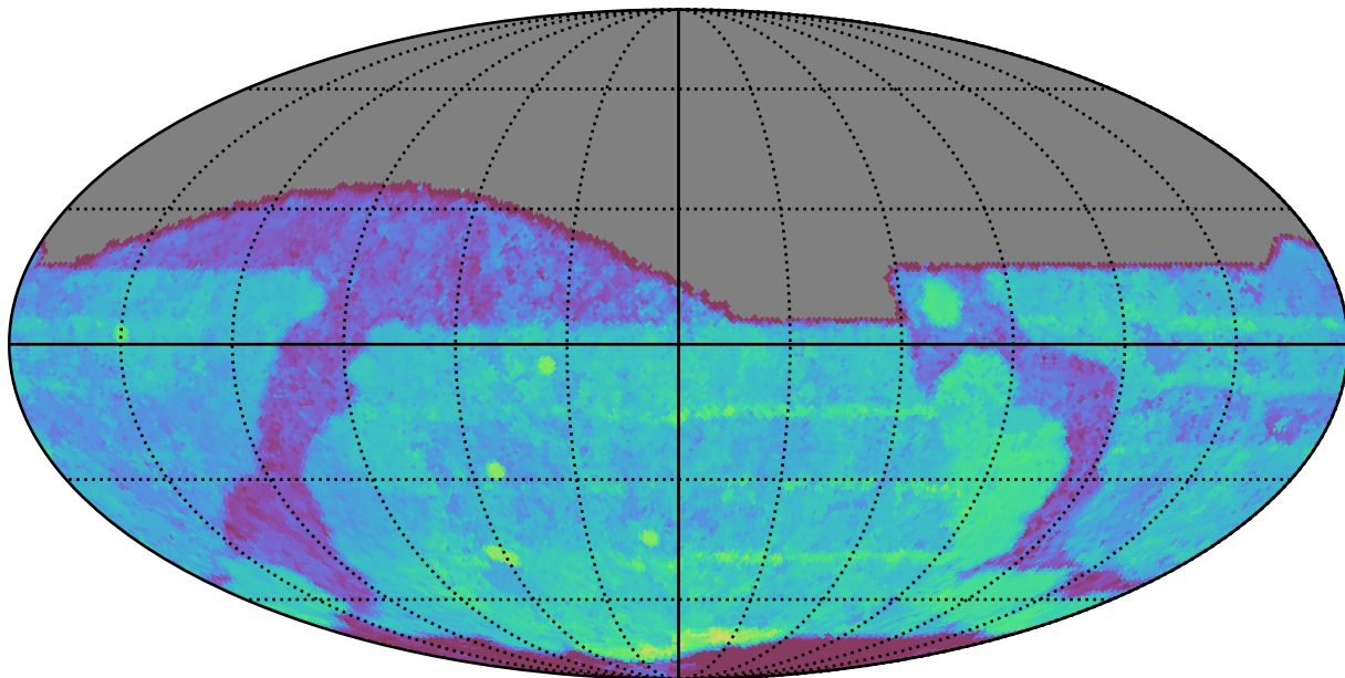
too_elab_r8_d3_griz_v3.4_10yrs All sky r band: Median Season Length
