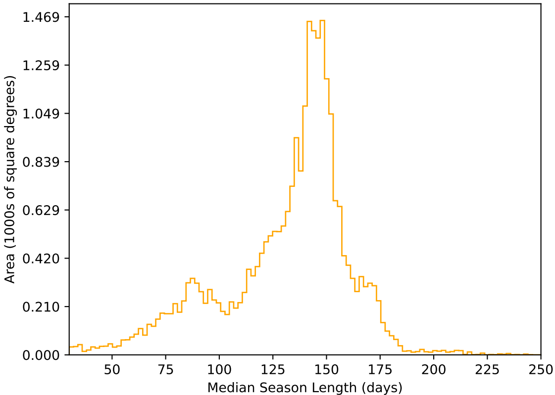
too_elab_r8_d3_griz_v3.4_10yrs All sky r band: Median Season Length
