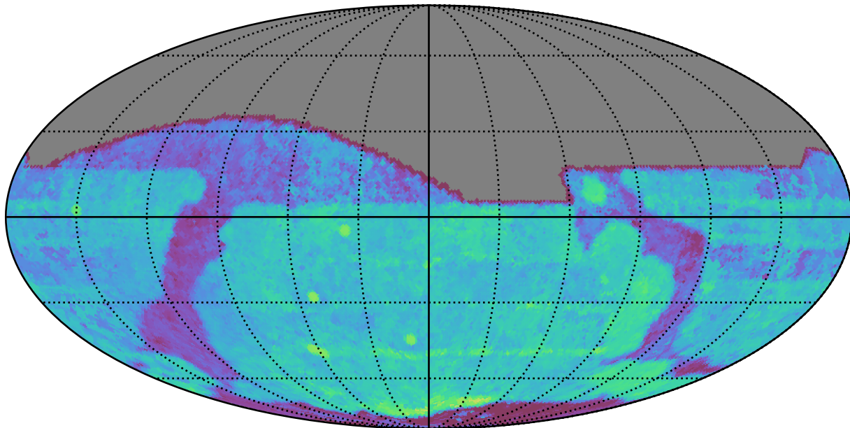
too_elab_r8_d3_griz_v3.4_10yrs All sky i band: Median Season Length
