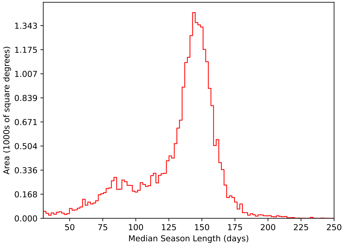
too_elab_r8_d3_griz_v3.4_10yrs All sky i band: Median Season Length
