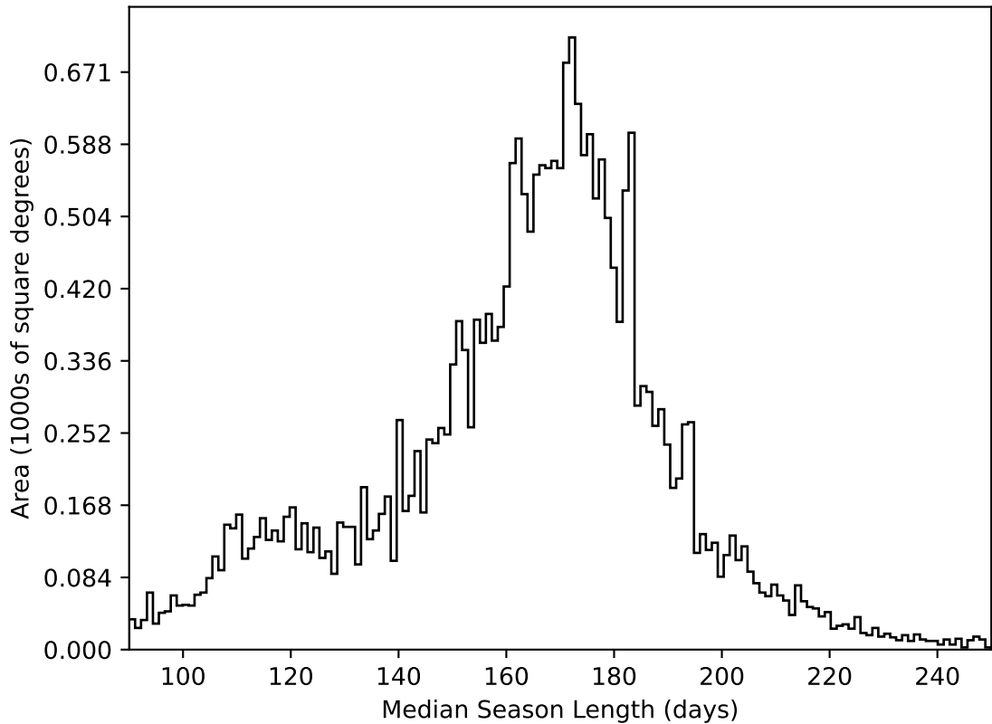
too_elab_r8_d3_griz_v3.4_10yrs All sky all bands: Median Season Length
