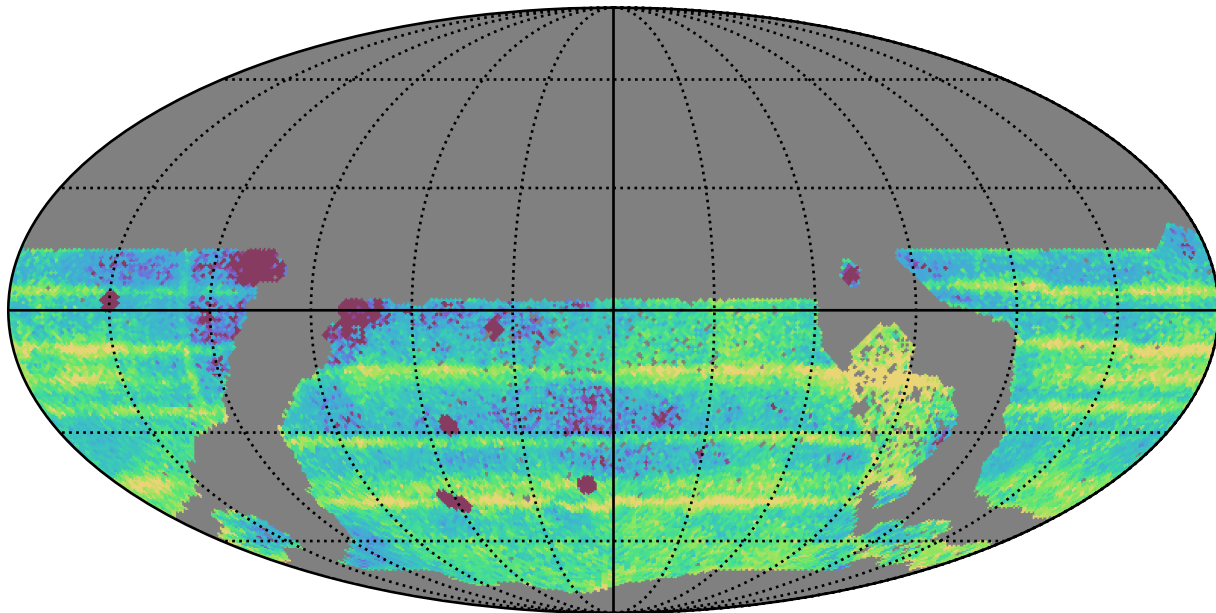
too_elab_r8_d3_griz_v3.4_10yrs WFD: Median Intra-Night Gap
