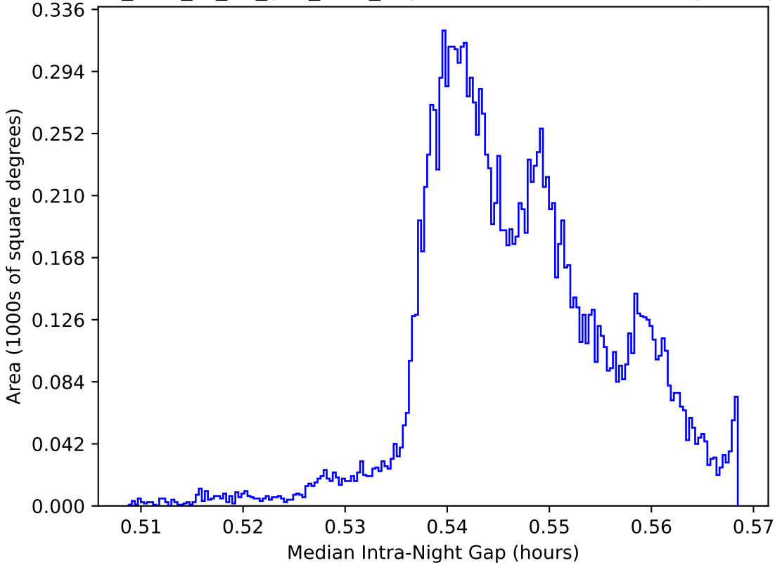
too_elab_r8_d3_griz_v3.4_10yrs WFD: Median Intra-Night Gap
