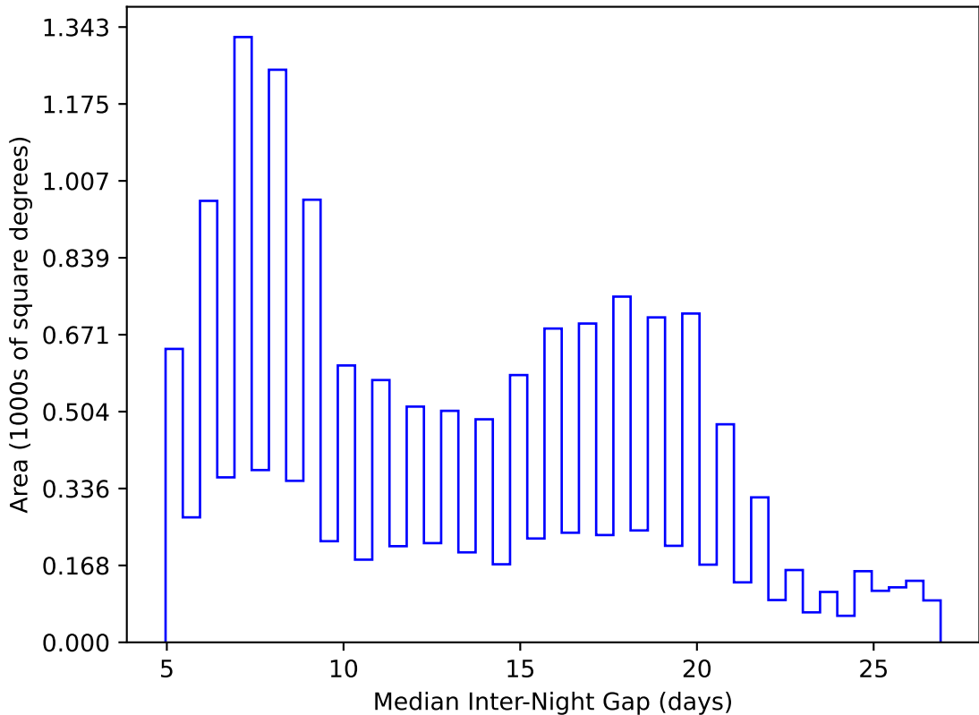
too_elab_r8_d3_griz_v3.4_10yrs WFD y band: Median Inter-Night Gap
