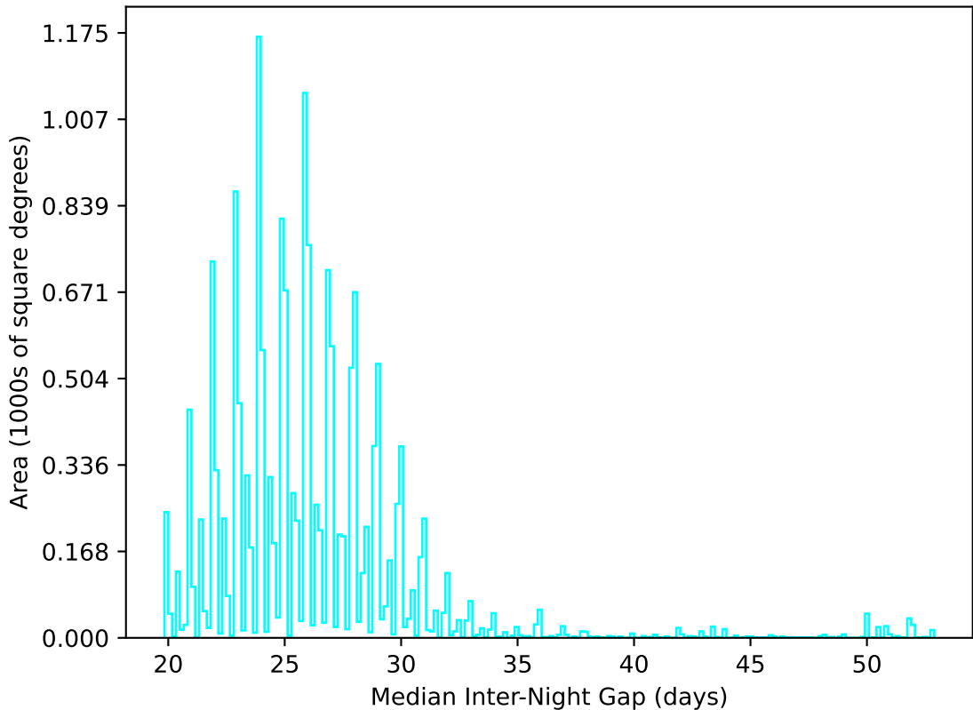
too_elab_r8_d3_griz_v3.4_10yrs WFD u band: Median Inter-Night Gap
