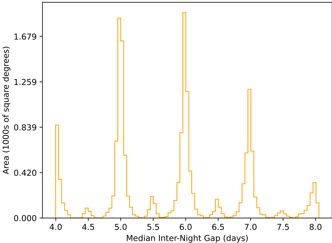
too_elab_r8_d3_griz_v3.4_10yrs WFD r band: Median Inter-Night Gap
