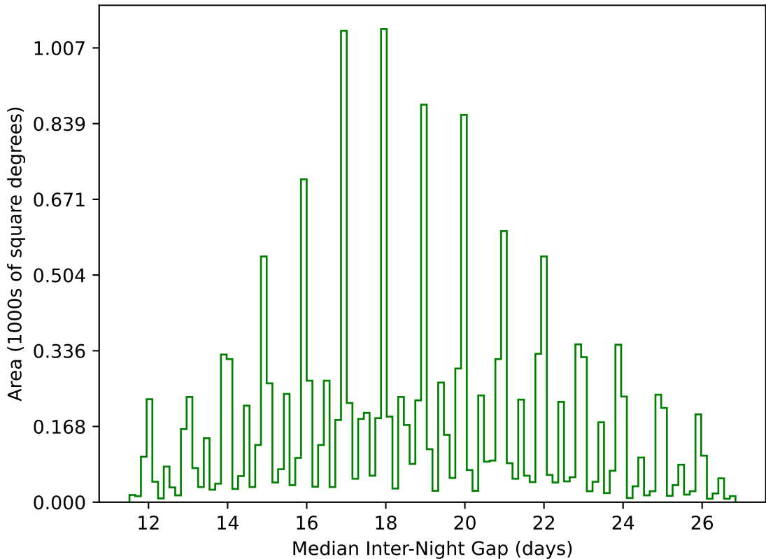
too_elab_r8_d3_griz_v3.4_10yrs WFD g band: Median Inter-Night Gap
