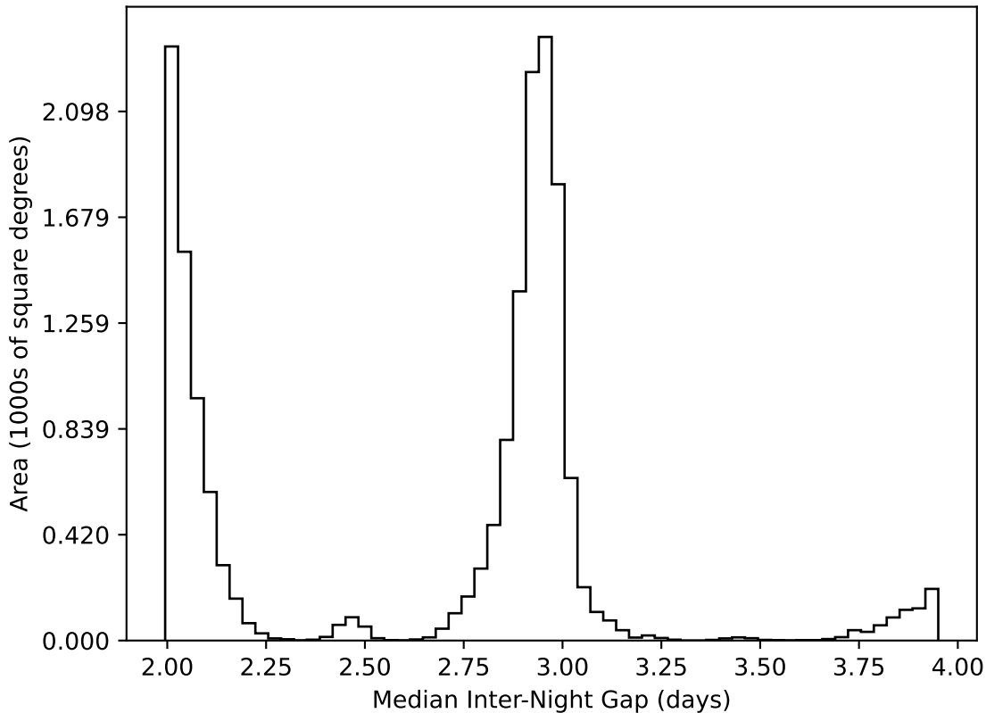
too_elab_r8_d3_griz_v3.4_10yrs WFD all bands: Median Inter-Night Gap
