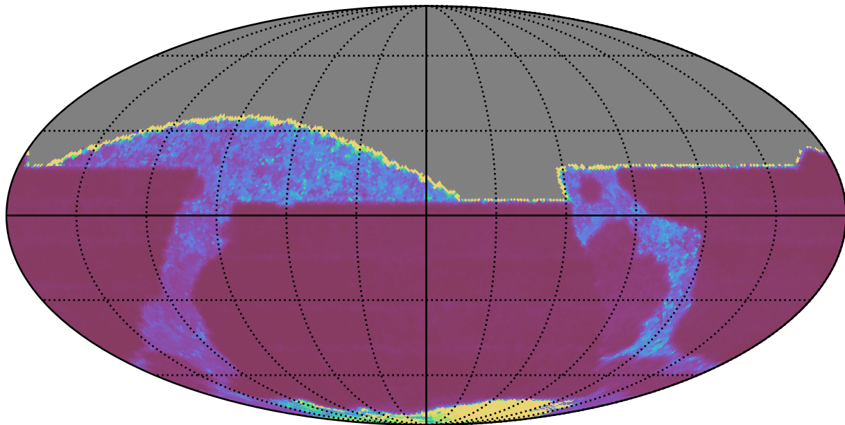
too_elab_r8_d3_griz_v3.4_10yrs All sky z band: Median Inter-Night Gap
