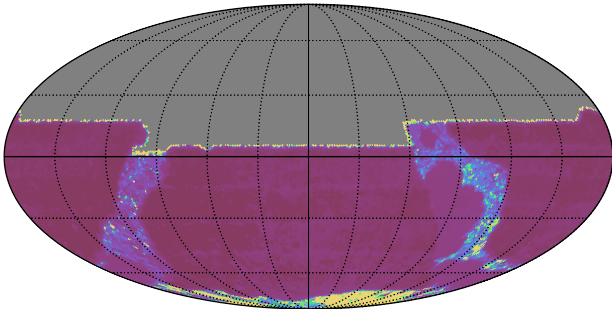
too_elab_r8_d3_griz_v3.4_10yrs All sky y band: Median Inter-Night Gap
