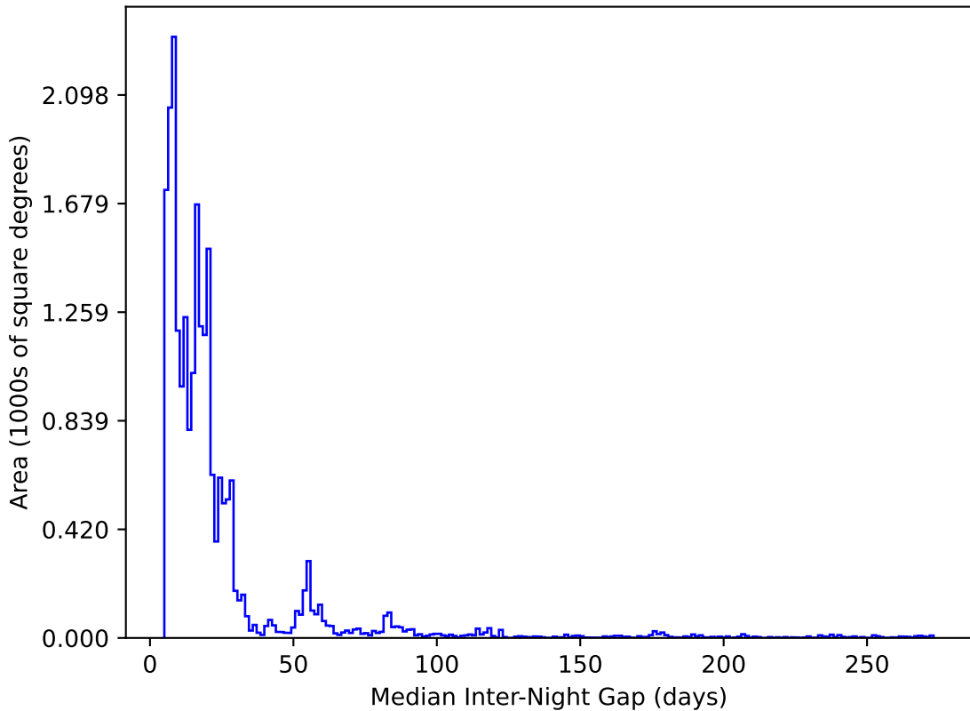
too_elab_r8_d3_griz_v3.4_10yrs All sky y band: Median Inter-Night Gap
