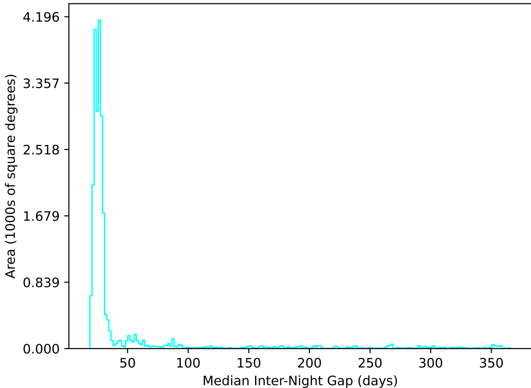
too_elab_r8_d3_griz_v3.4_10yrs All sky u band: Median Inter-Night Gap
