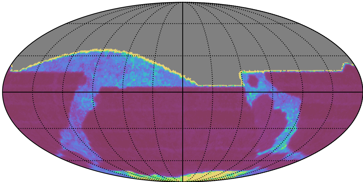
too_elab_r8_d3_griz_v3.4_10yrs All sky i band: Median Inter-Night Gap
