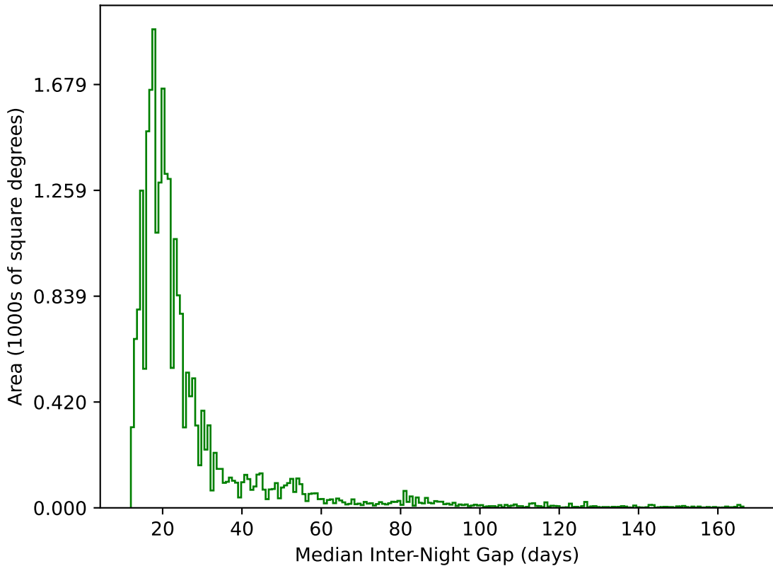
too_elab_r8_d3_griz_v3.4_10yrs All sky g band: Median Inter-Night Gap
