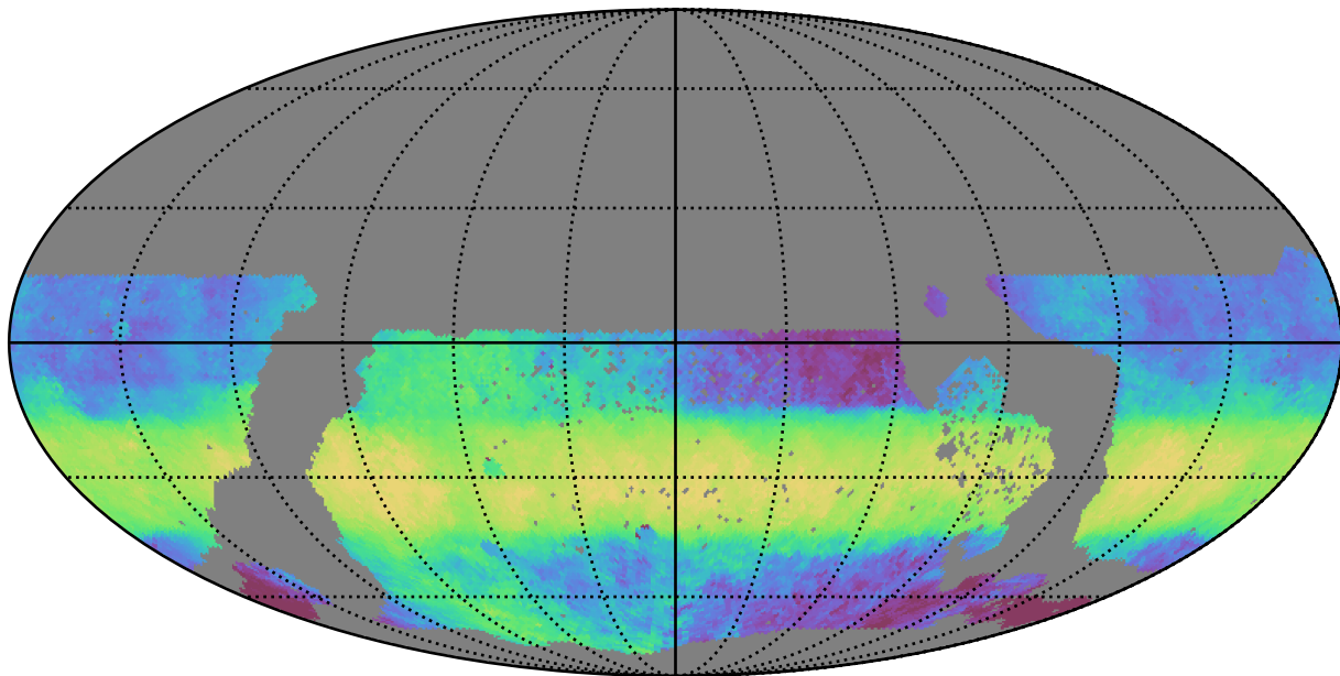
too_elab_r8_d3_griz_v3.4_10yrs WFD z band: Median HA
