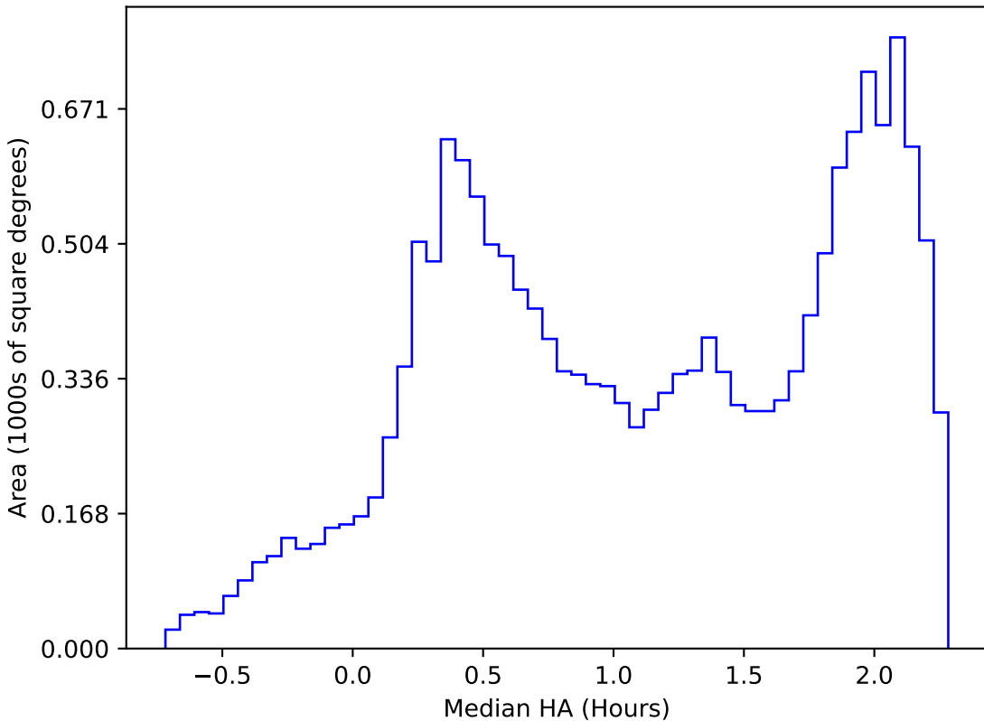
too_elab_r8_d3_griz_v3.4_10yrs WFD z band: Median HA
