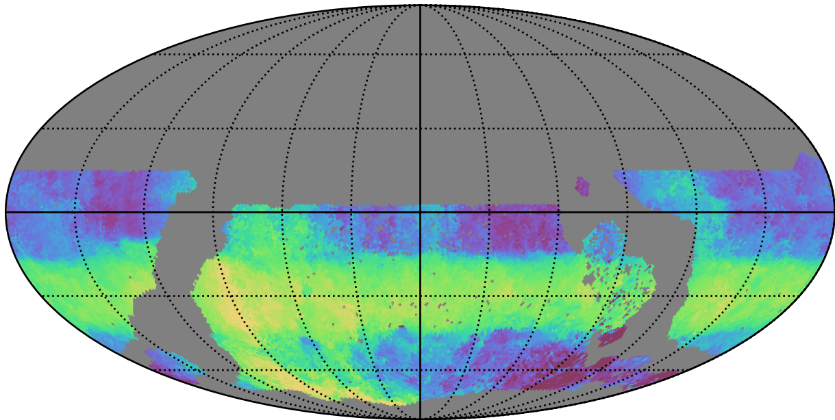
too_elab_r8_d3_griz_v3.4_10yrs WFD u band: Median HA
