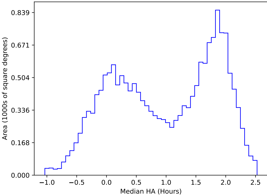
too_elab_r8_d3_griz_v3.4_10yrs WFD u band: Median HA
