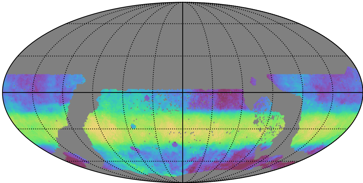
too_elab_r8_d3_griz_v3.4_10yrs WFD i band: Median HA
