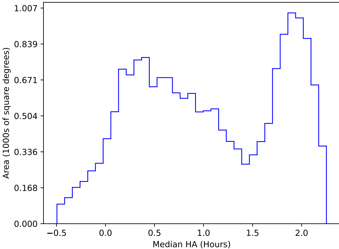
too_elab_r8_d3_griz_v3.4_10yrs WFD i band: Median HA
