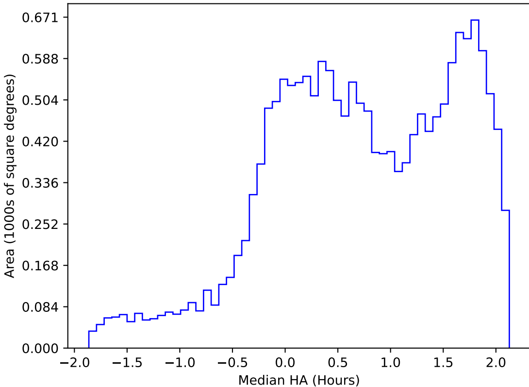
too_elab_r8_d3_griz_v3.4_10yrs WFD g band: Median HA
