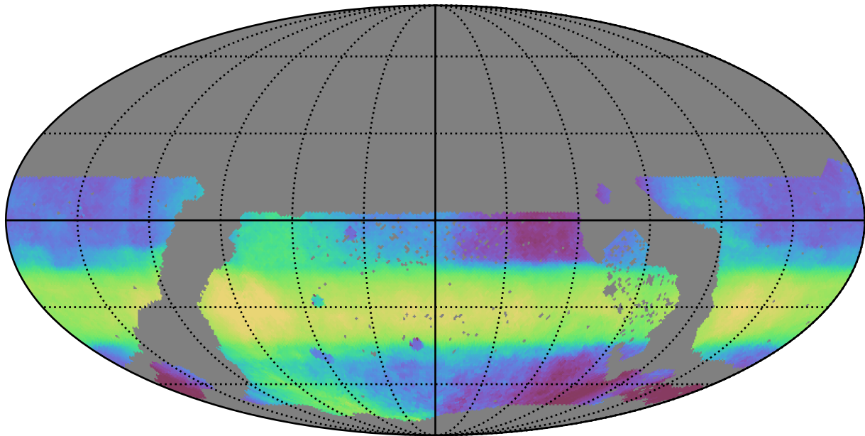
too_elab_r8_d3_griz_v3.4_10yrs WFD all bands: Median HA
