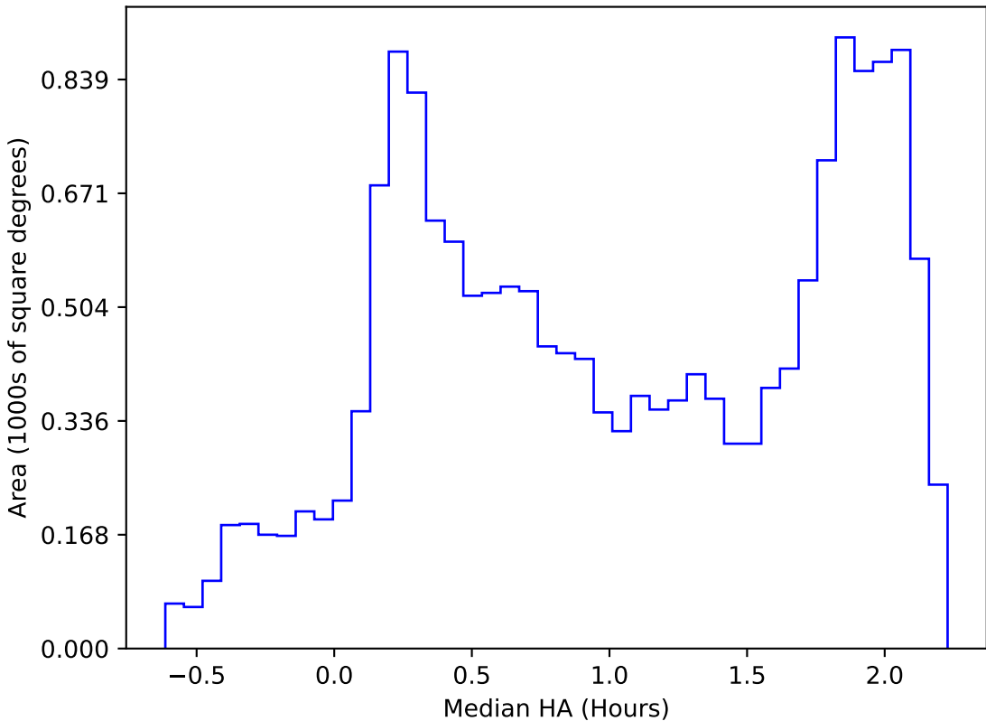
too_elab_r8_d3_griz_v3.4_10yrs WFD all bands: Median HA
