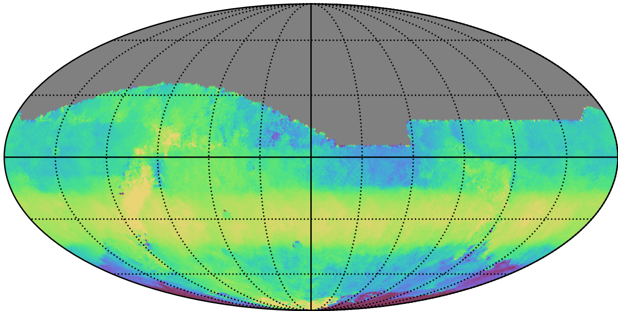
too_elab_r8_d3_griz_v3.4_10yrs All sky z band: Median HA
