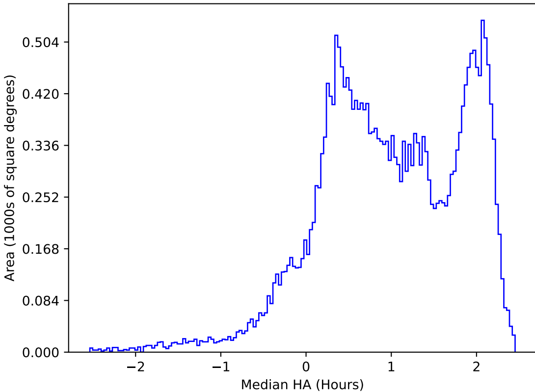
too_elab_r8_d3_griz_v3.4_10yrs All sky z band: Median HA
