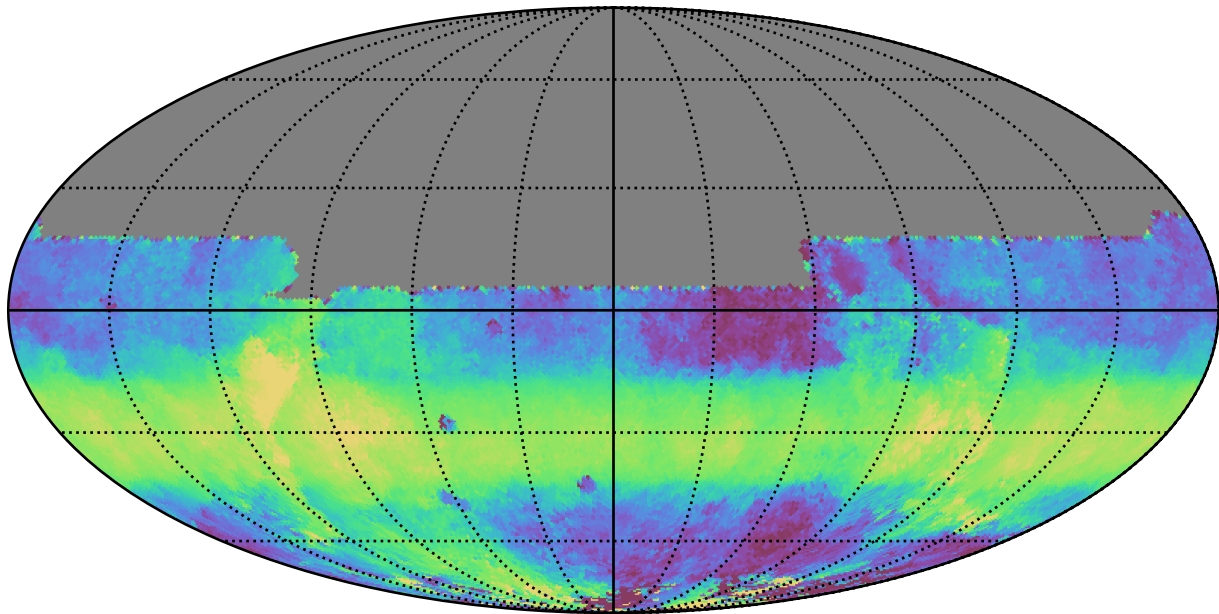
too_elab_r8_d3_griz_v3.4_10yrs All sky y band: Median HA
