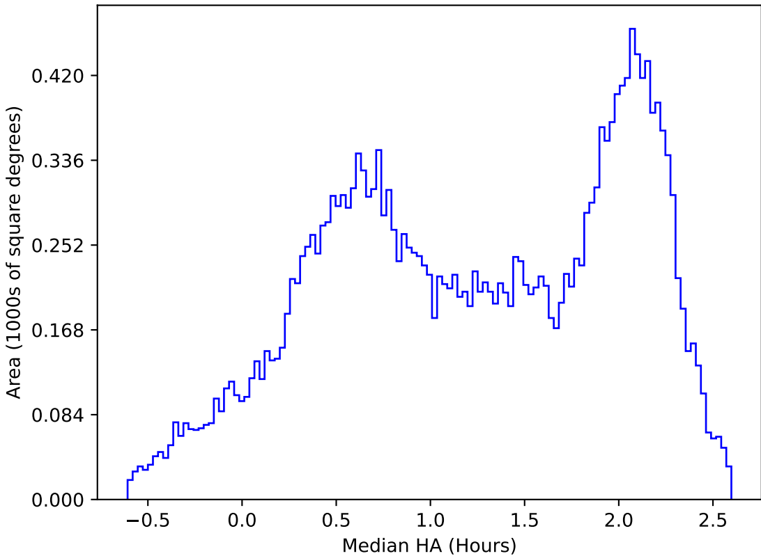
too_elab_r8_d3_griz_v3.4_10yrs All sky y band: Median HA
