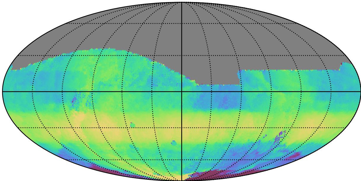
too_elab_r8_d3_griz_v3.4_10yrs All sky r band: Median HA
