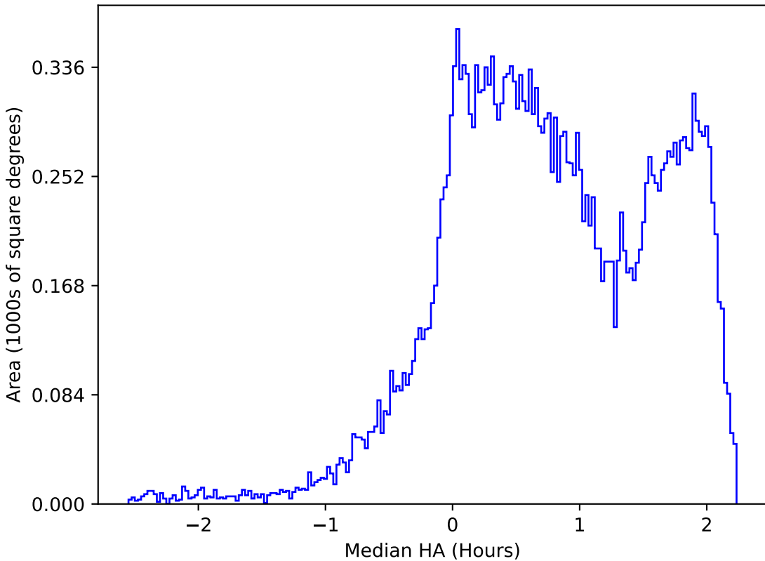
too_elab_r8_d3_griz_v3.4_10yrs All sky r band: Median HA
