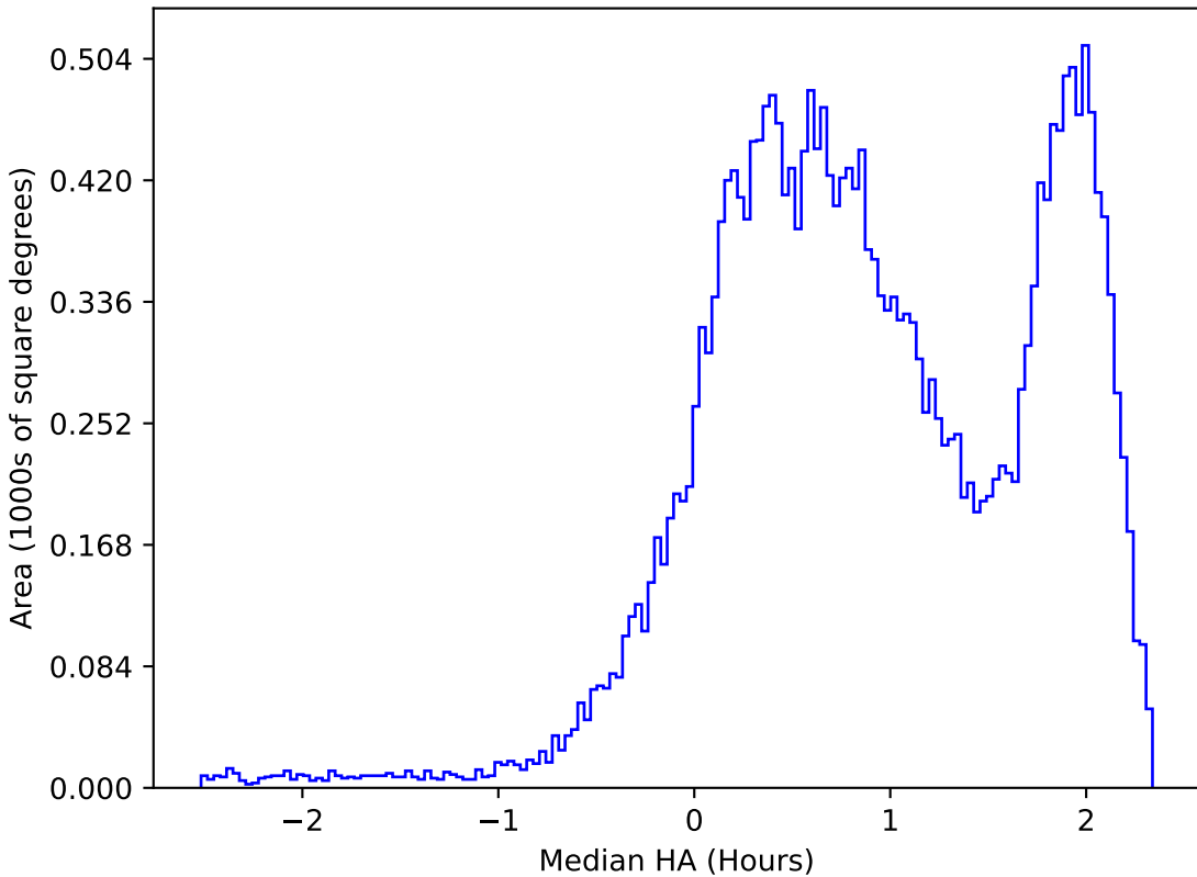
too_elab_r8_d3_griz_v3.4_10yrs All sky i band: Median HA
