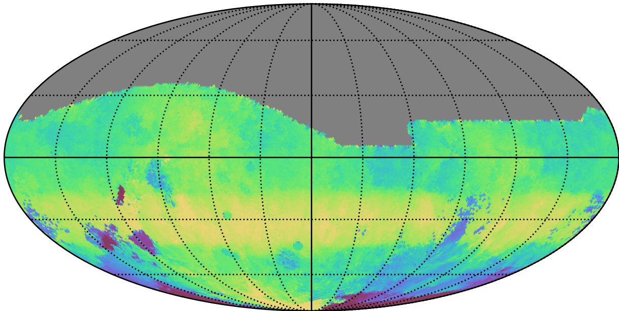
too_elab_r8_d3_griz_v3.4_10yrs All sky g band: Median HA
