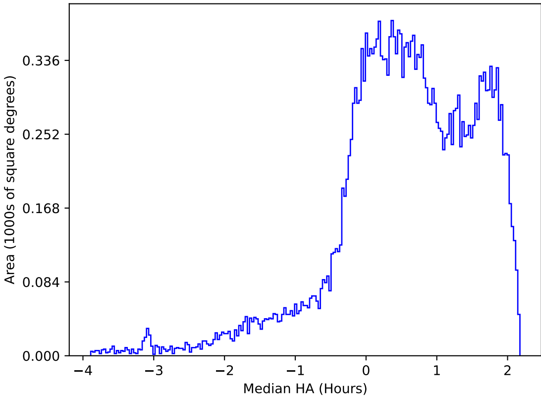
too_elab_r8_d3_griz_v3.4_10yrs All sky g band: Median HA
