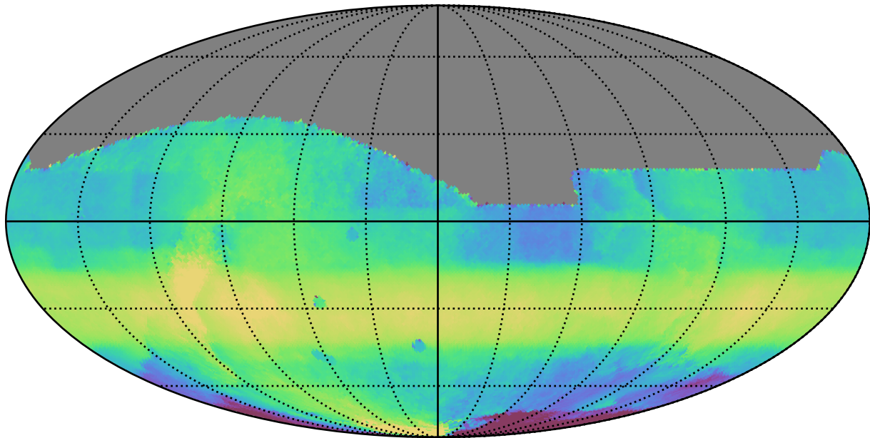
too_elab_r8_d3_griz_v3.4_10yrs All sky all bands: Median HA
