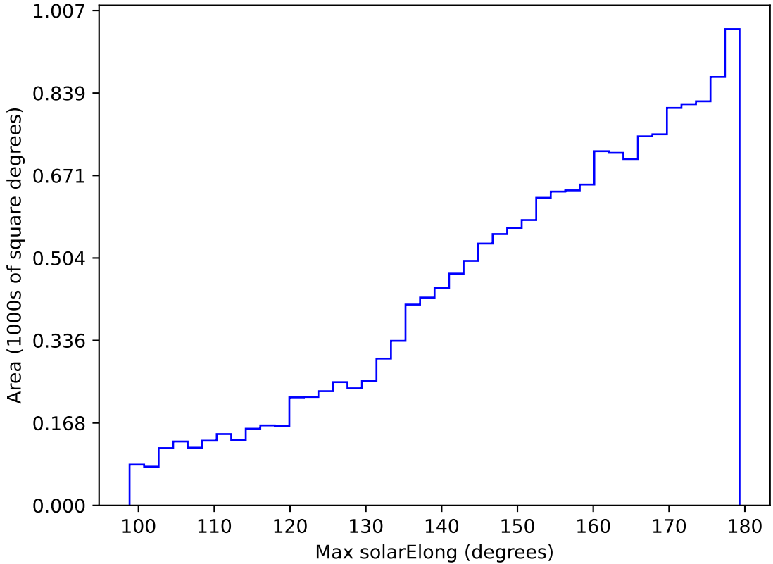
too_elab_r8_d3_griz_v3.4_10yrs WFD y band: Max solarElong
