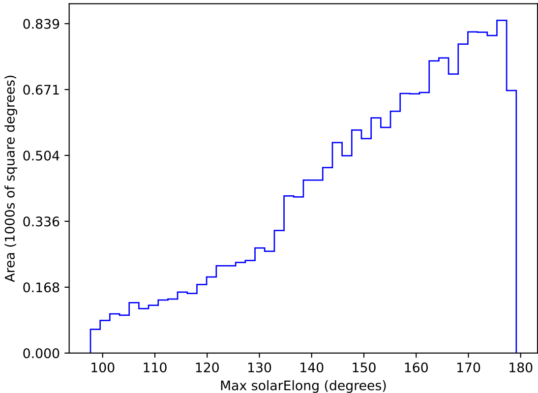
too_elab_r8_d3_griz_v3.4_10yrs WFD u band: Max solarElong
