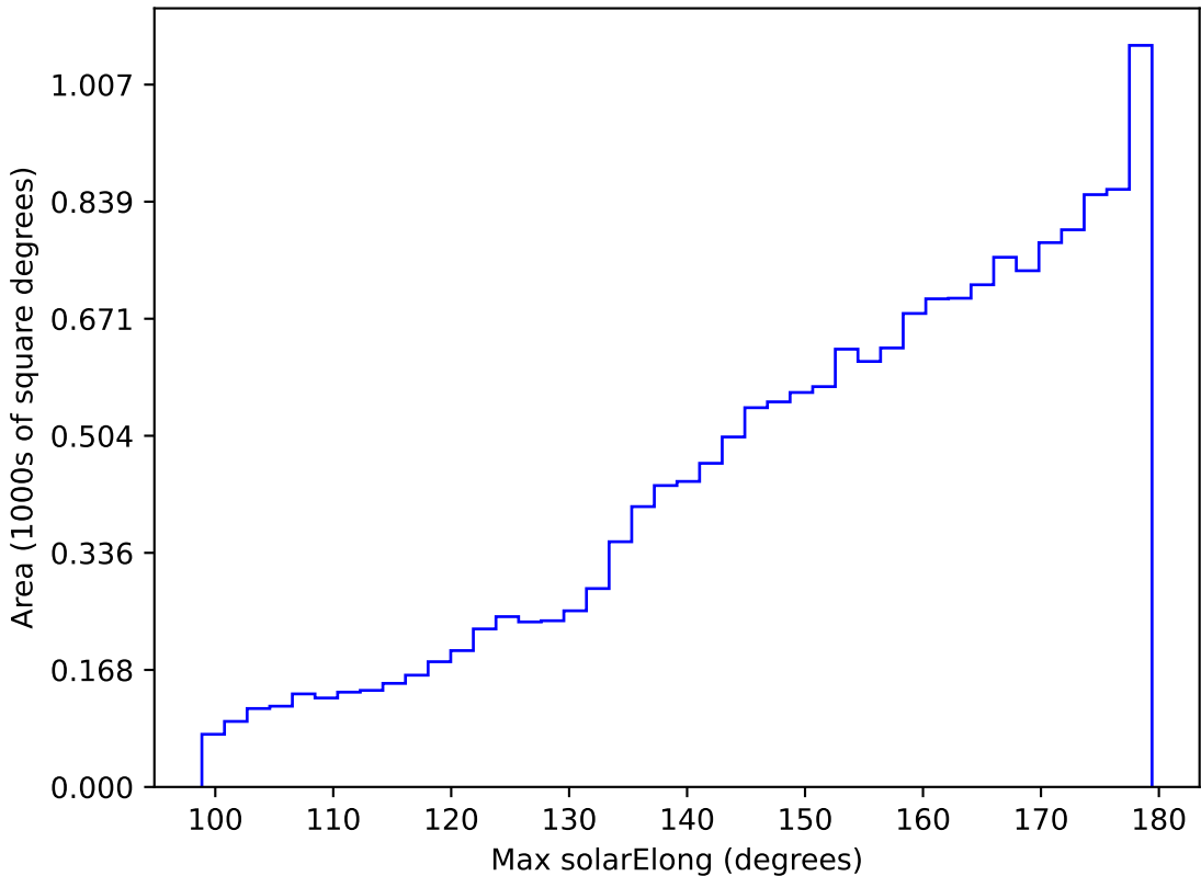
too_elab_r8_d3_griz_v3.4_10yrs WFD r band: Max solarElong
