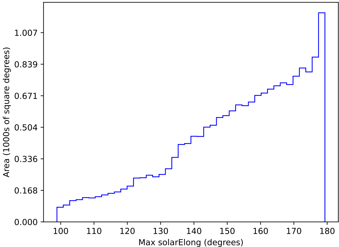
too_elab_r8_d3_griz_v3.4_10yrs WFD i band: Max solarElong
