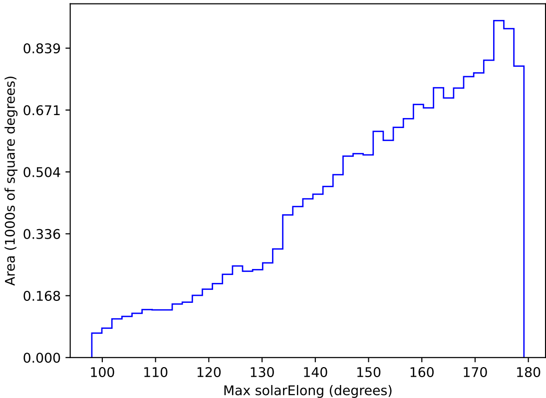
too_elab_r8_d3_griz_v3.4_10yrs WFD g band: Max solarElong
