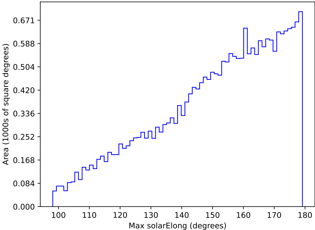
too_elab_r8_d3_griz_v3.4_10yrs All sky y band: Max solarElong
