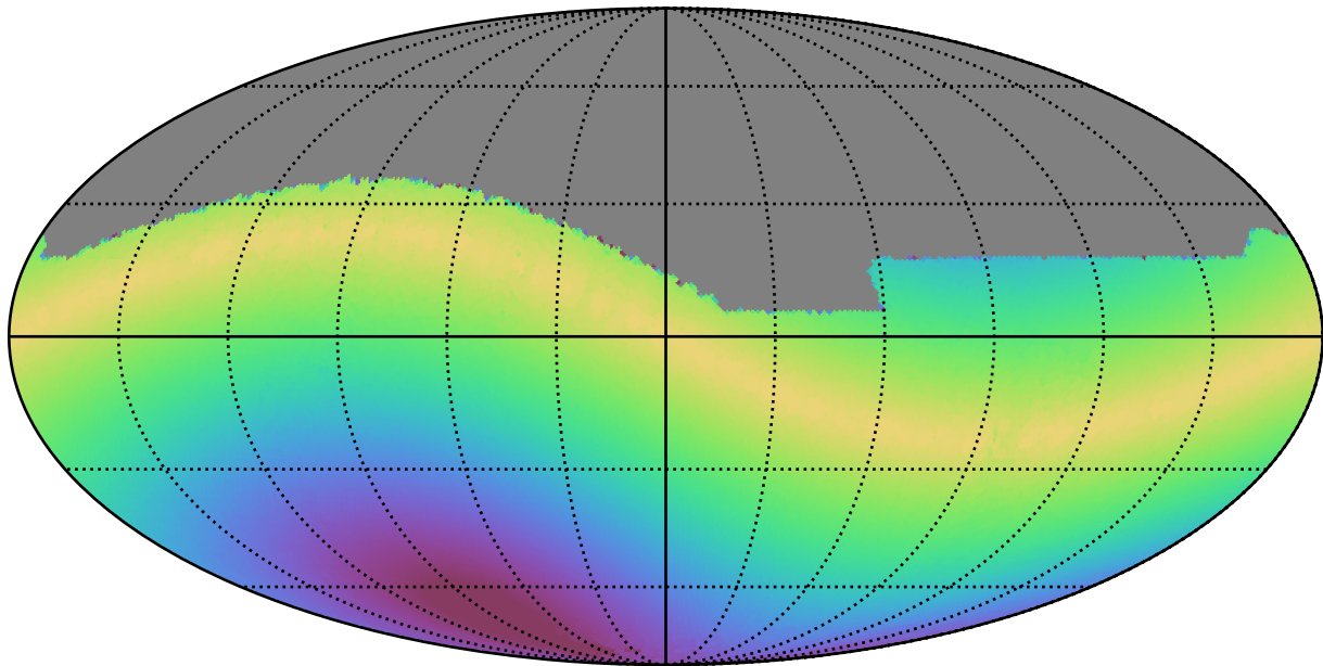
too_elab_r8_d3_griz_v3.4_10yrs All sky i band: Max solarElong
