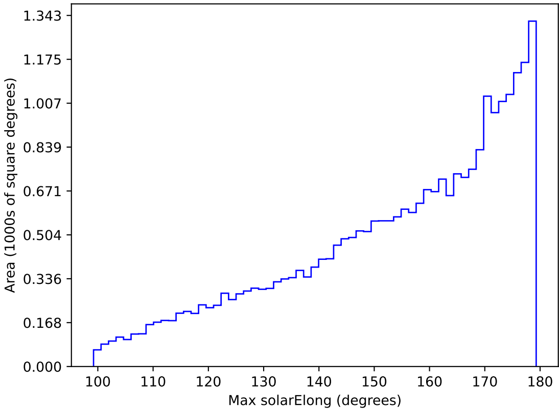
too_elab_r8_d3_griz_v3.4_10yrs All sky i band: Max solarElong
