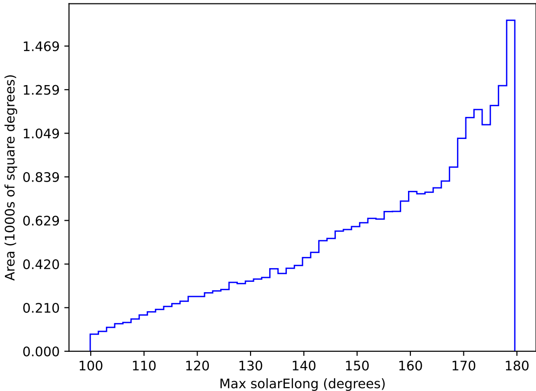
too_elab_r8_d3_griz_v3.4_10yrs All sky all bands: Max solarElong
