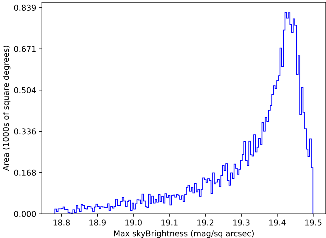
too_elab_r8_d3_griz_v3.4_10yrs Yr 1 z band: Max skyBrightness
