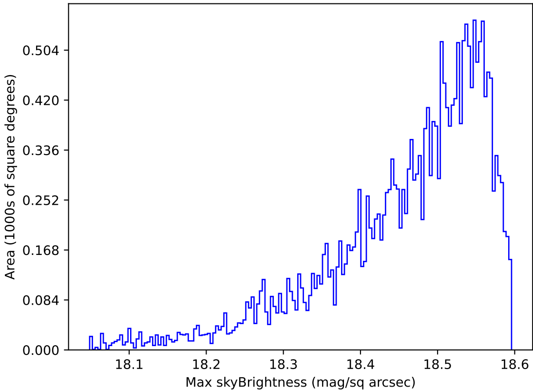
too_elab_r8_d3_griz_v3.4_10yrs Yr 1 y band: Max skyBrightness
