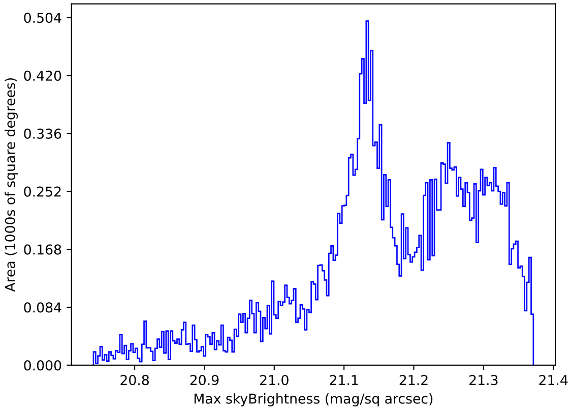
too_elab_r8_d3_griz_v3.4_10yrs Yr 1 r band: Max skyBrightness
